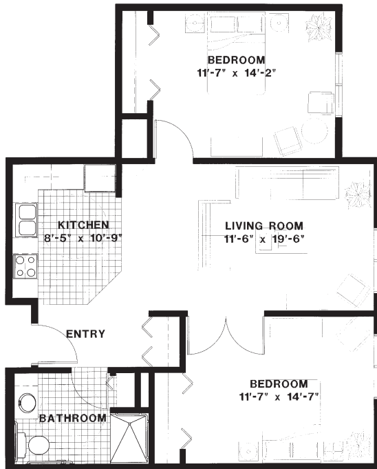
UNIT L TWO BEDROOM
