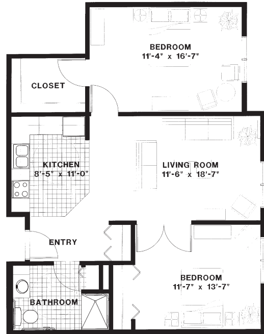
UNIT H TWO BEDROOM
