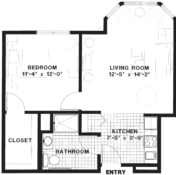
UNIT C ONE BEDROOM
