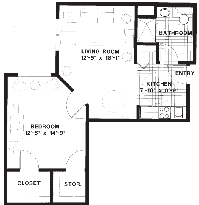
UNIT D ONE BEDROOM
